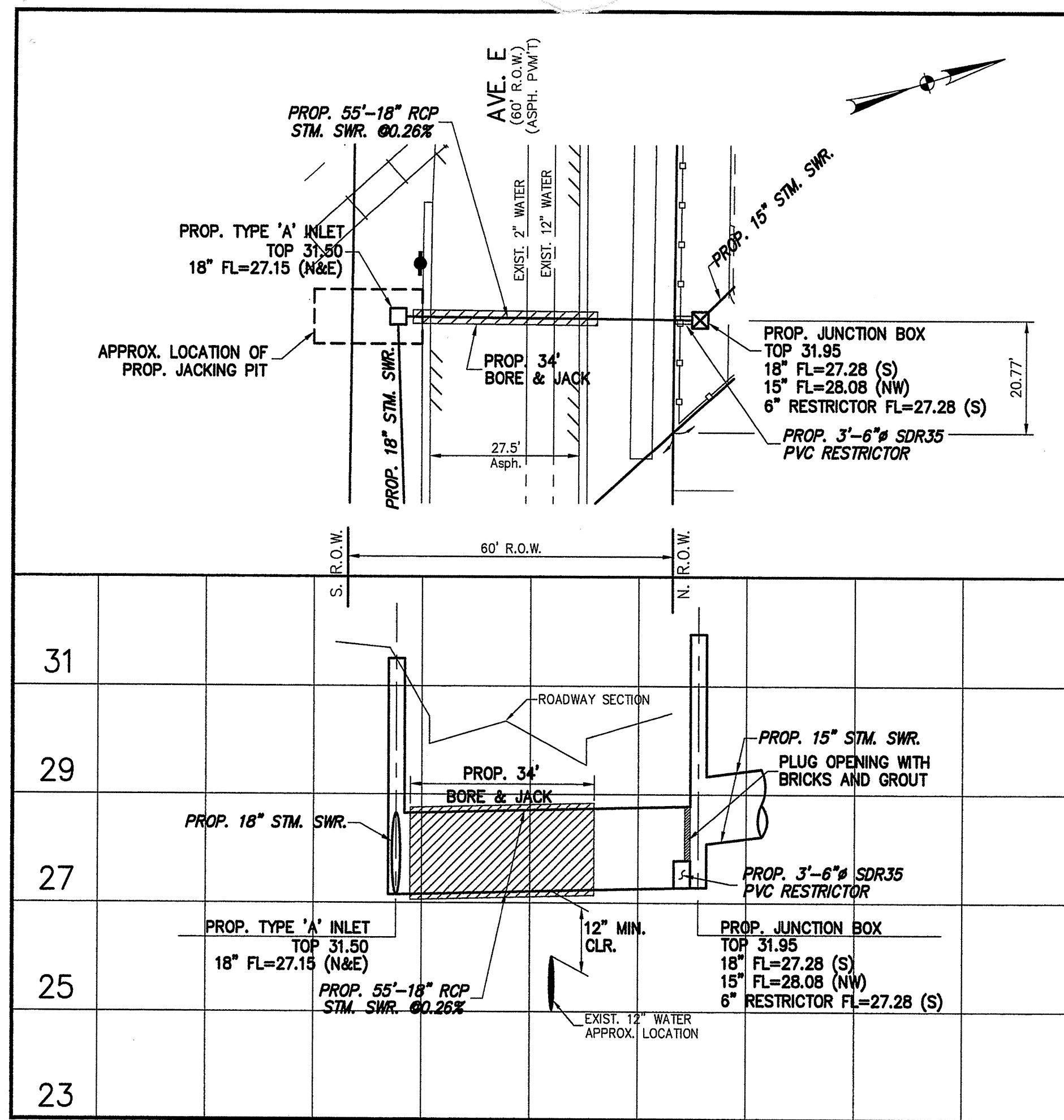
PLAN & PROFILE FOR PROP. 15" STORM RCP
