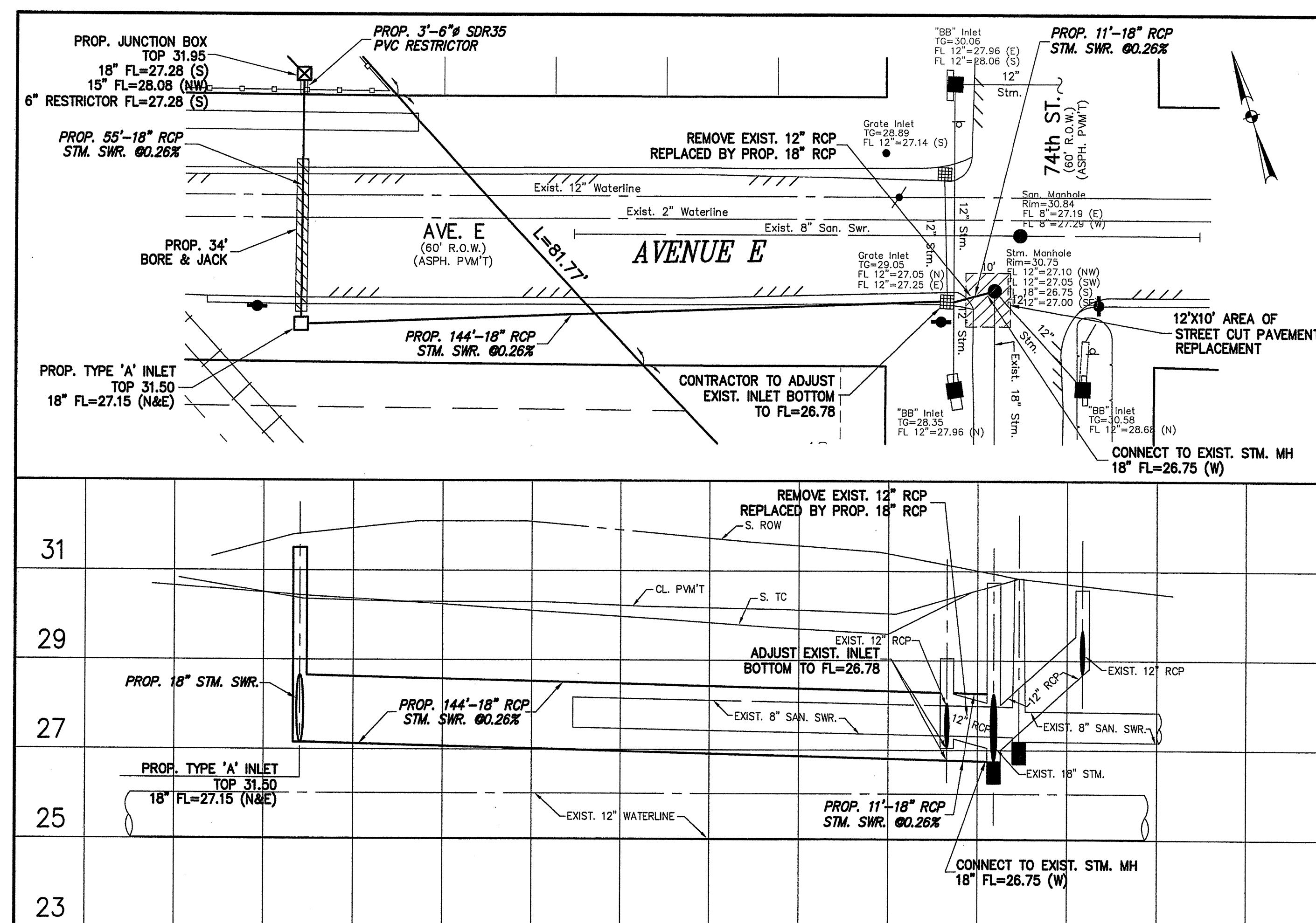
PLAN & PROFILE FOR PROP. 18" STORM RCP
