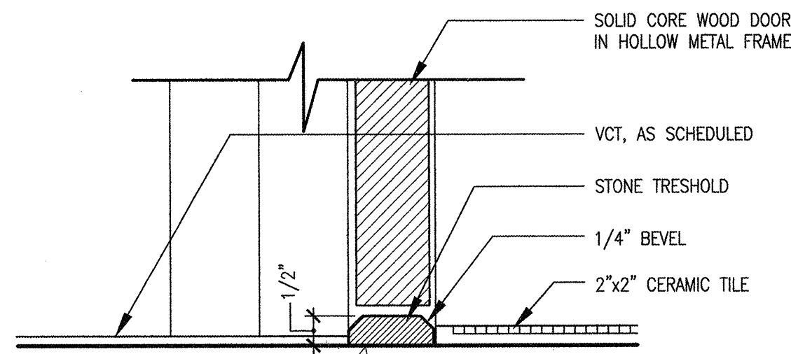
VCT TO CERAMIC TILE DETAIL (12)
