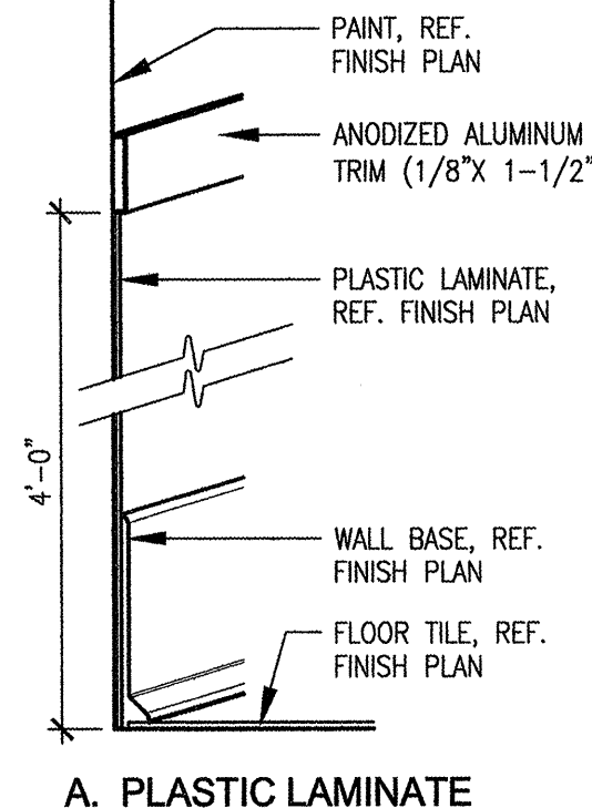
WALL TRANSITION DETAILS (10)
