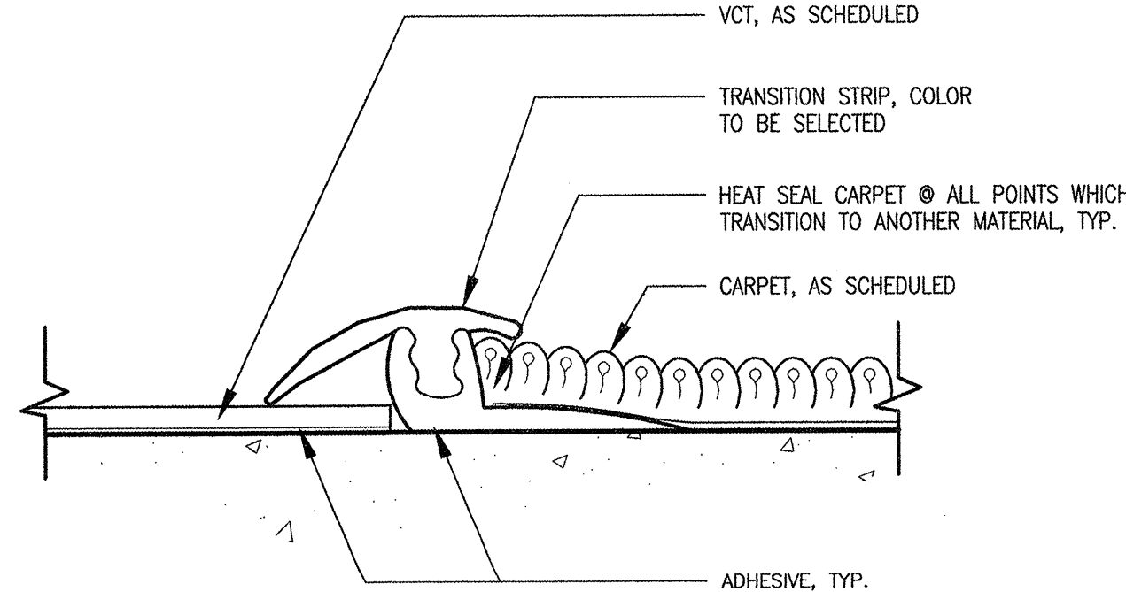
CARPET TO VCT DETAIL (11)
